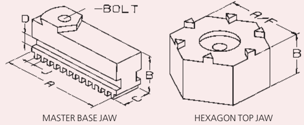
MASTER BASE JAW
