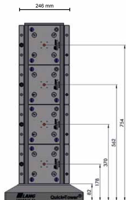
Tower 70850, height 860 max. 4 pallets on each side
