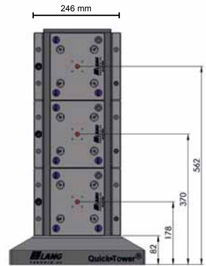
Tower 70650, height 668 max. 3 pallets on each side
