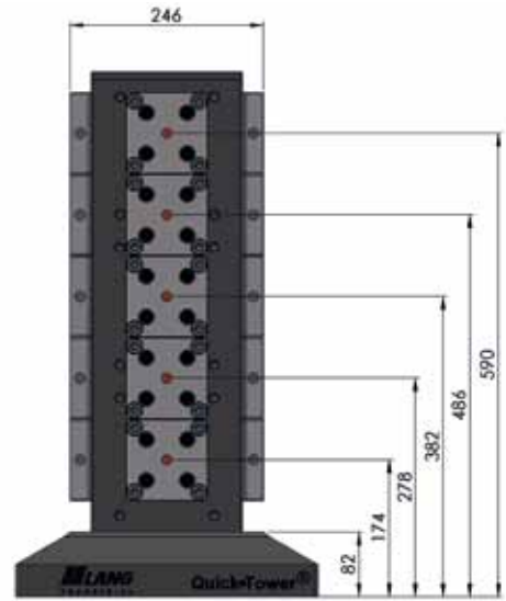
Tower 70650, height 668 max. 5 pallets on each side
