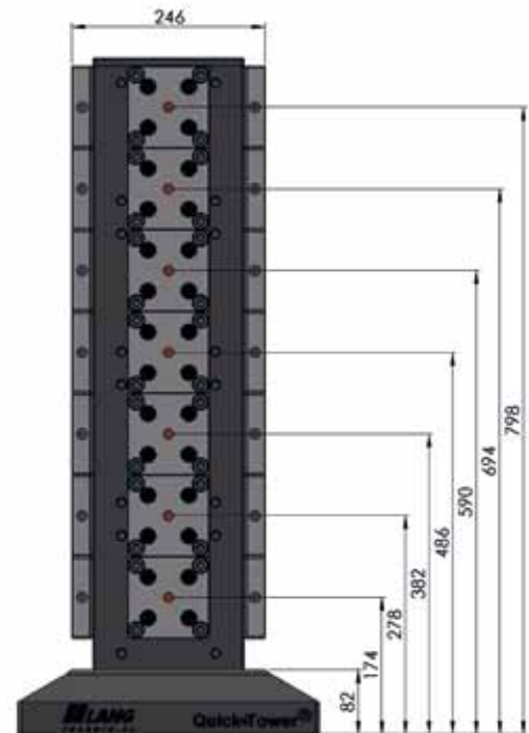
Tower 70850, height 860 max. 7 pallets on each side
